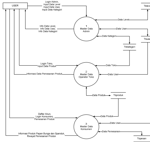
Gambar 3 Data Flow Diagram Level 1
