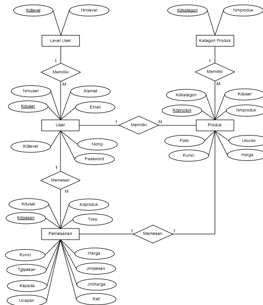
Gambar 1 Entity Relationship Diagram (ERD)
